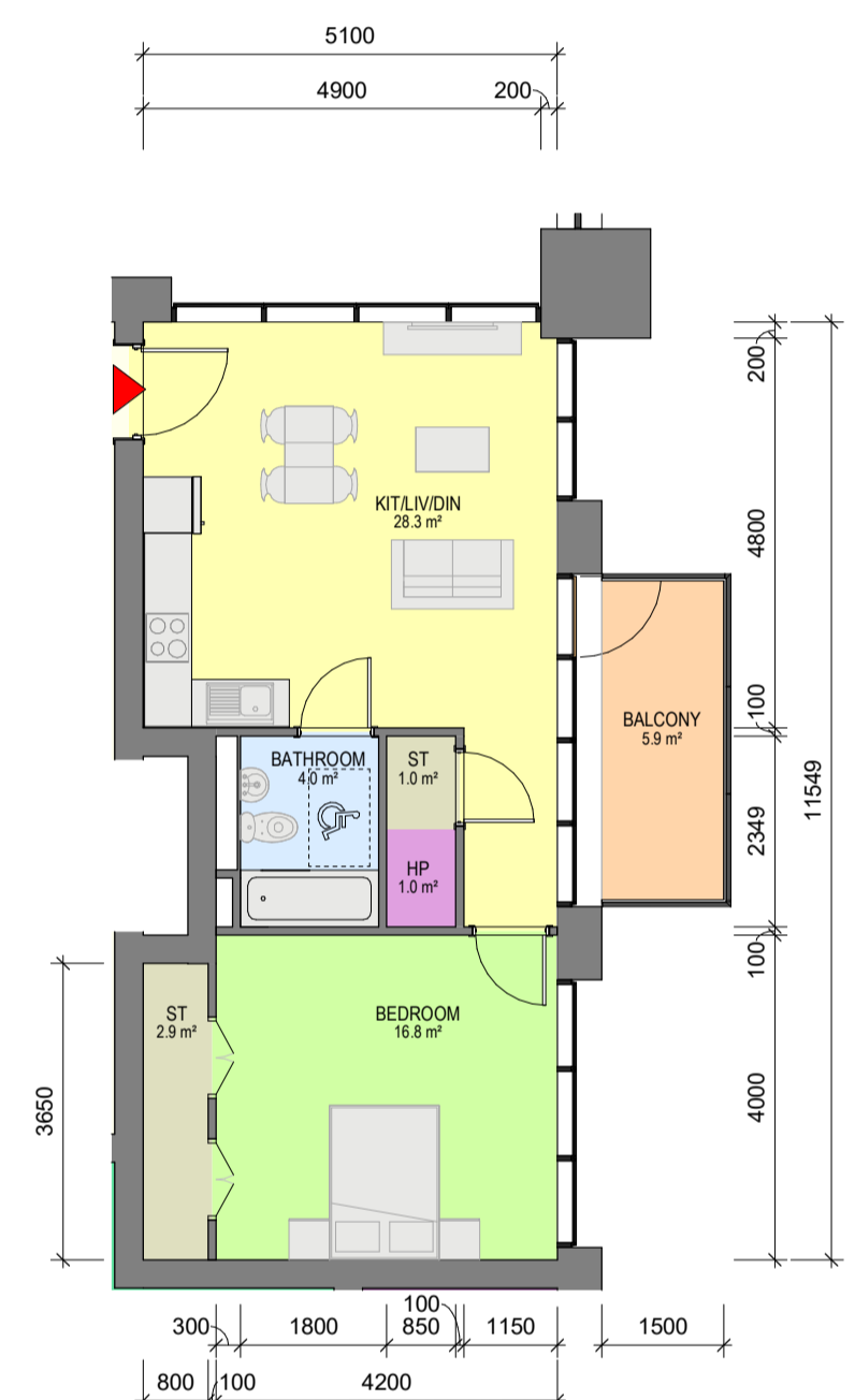
10 Apartment Type 1AN 1 : 100 - 1 BED, 2 PERSON APARTMENT - NET INTERNAL AREA (NIA) Areas shown in plan - GROSS INTERNAL AREA (GIA) : 56.25sqm
