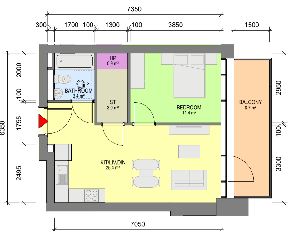
3 Apartment Type 1AG 1 : 100 - 1 BED, 2 PERSON APARTMENT - NET INTERNAL AREA (NIA) Areas shown in plan - GROSS INTERNAL AREA (GIA) : 45.99sqm
