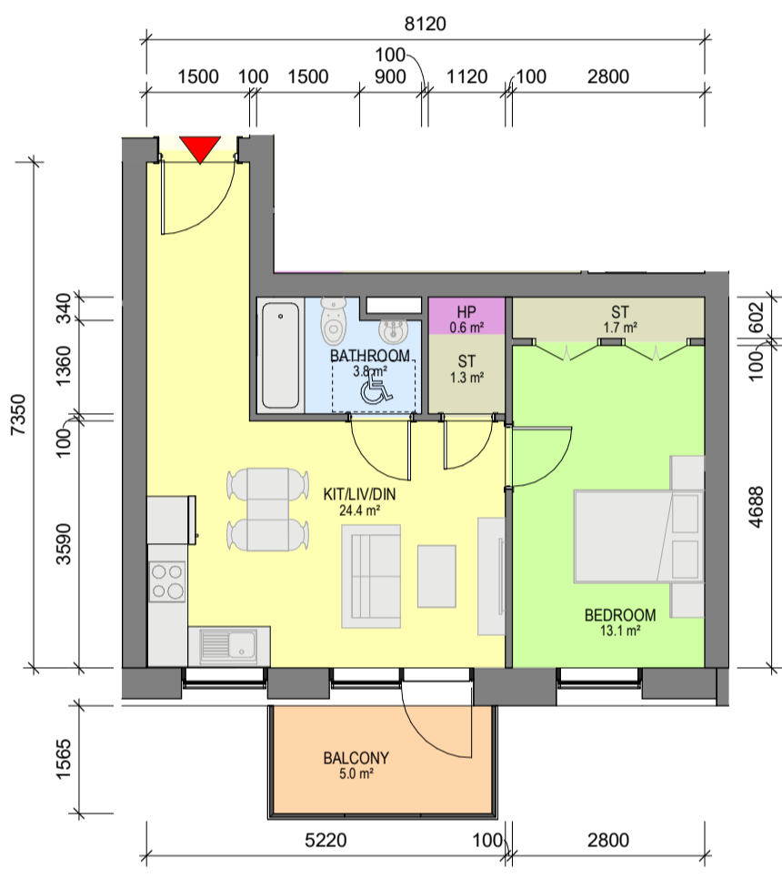
7 Apartment Type 1AK 1 : 100 - 1 BED, 2 PERSON APARTMENT - NET INTERNAL AREA (NIA) Areas shown in plan - GROSS INTERNAL AREA (GIA) : 46.69sqm
