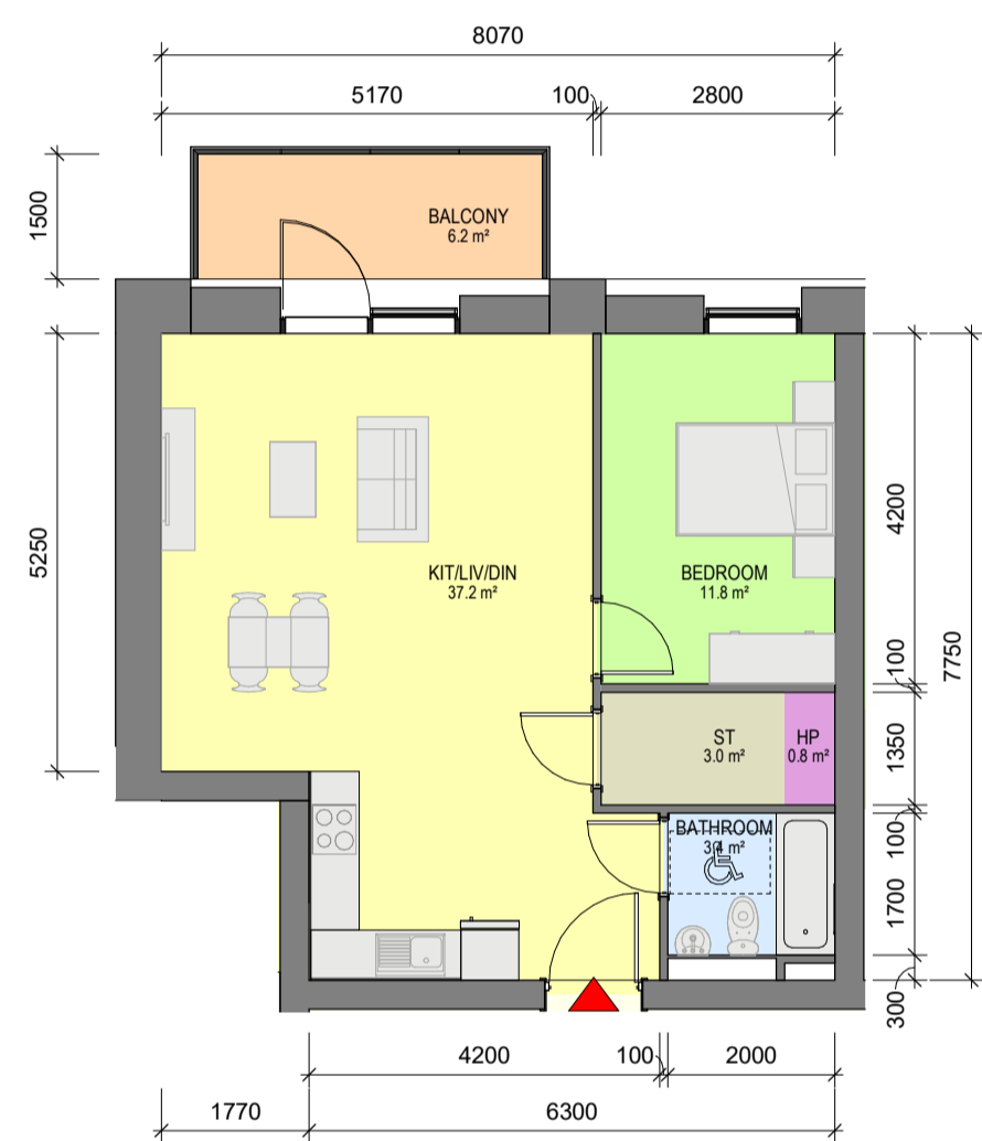
6 Apartment Type 1AJ 1 : 100 - 1 BED, 2 PERSON APARTMENT - NET INTERNAL AREA (NIA) Areas shown in plan - GROSS INTERNAL AREA (GIA) : 58.12sqm
