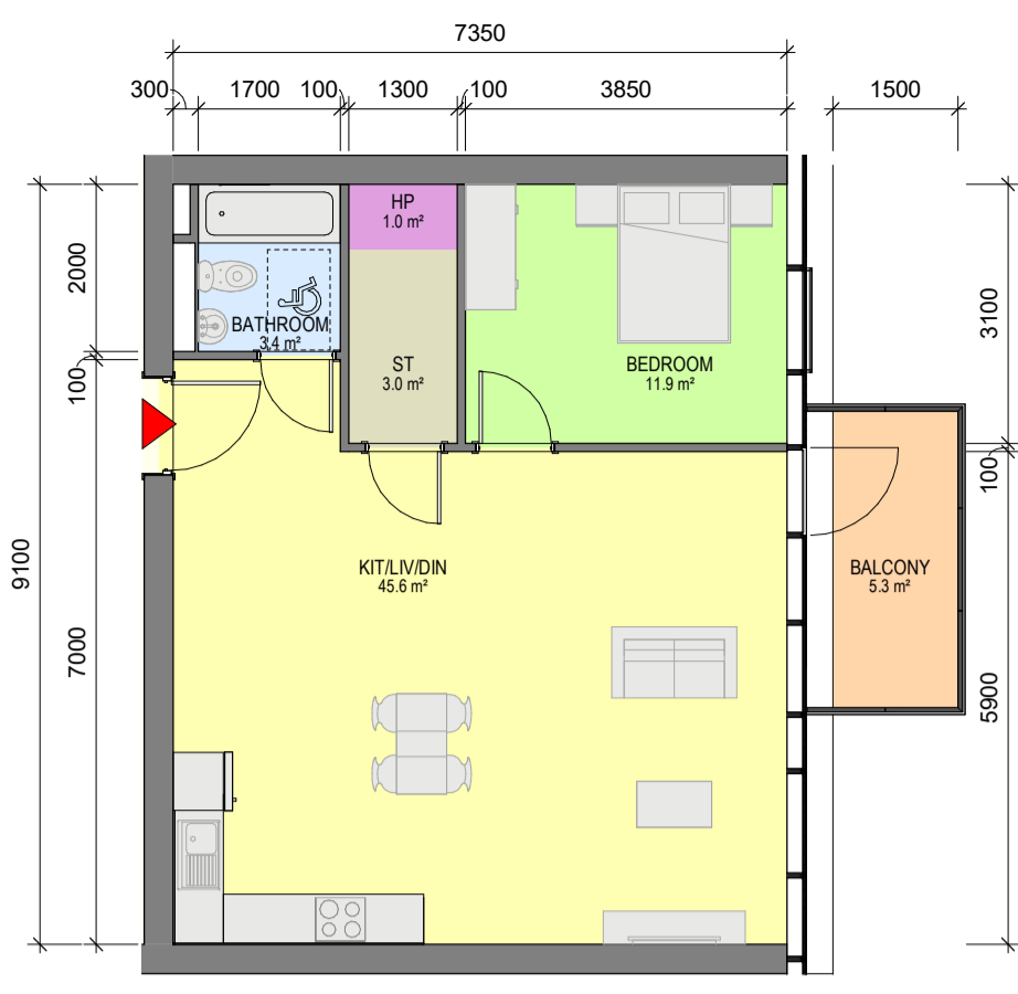
4 Apartment Type 1AH 1 : 100 - 1 BED, 2 PERSON APARTMENT - NET INTERNAL AREA (NIA) Areas shown in plan - GROSS INTERNAL AREA (GIA) : 66.89sqm
